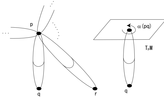
FIGURE 4. This is the picture of decomposition of the tangential representation on the fixed point p \in M^T .
