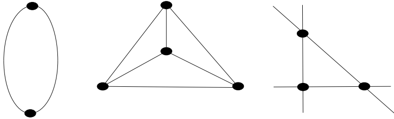
FIGURE 5. This is the picture of graphs. The left graph is the 2-valent graph with the multi-edge, the middle graph is the 3-valent graph, and the right graph is the 4-valent graph with 6 legs.
