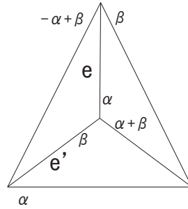
FIGURE 9. A (3, 2) -type GKM graph \mathcal{G}_2 with the connection \nabla^{(2)} , i.e., \nabla_e^{(2)} \neq \nabla_e^{st} and \nabla_{e'}^{(2)} \neq \nabla_{e'}^{st} . This axial function is nothing but the axial function of \mathcal{G}_0(1, 1) .
