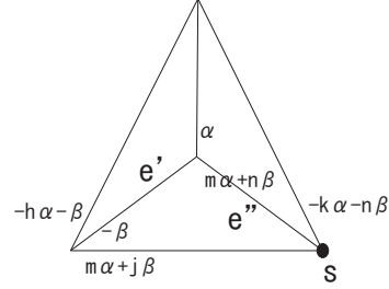
FIGURE 4. The axial functions around e', e'' .
