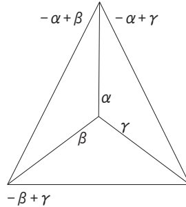
FIGURE 1. A (3,3)-type GKM graph \mathcal{G}_{st} . We omit the label on the different direction because it is determined automatically by the axiom (1).
