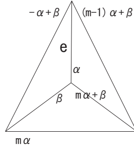
FIGURE 8. A (3, 2) -type GKM graph \mathcal{G}_1(m) ( m \in \mathbb{N} ) with the connection \nabla^{(1)} , i.e., \nabla_e^{(1)} \neq \nabla_e^{st} . This axial function is nothing but the axial function of \mathcal{G}_0(m, 1) .
