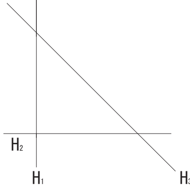
FIGURE 1. A hyperplane arrangement of T^*\mathbb{C}P(2)
