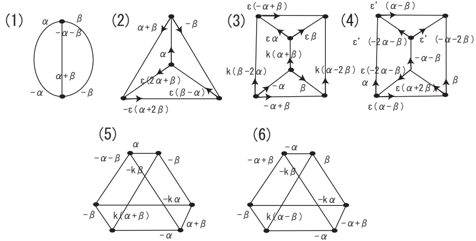
FIGURE 1. The list of complexity one GKM graphs with certain S_3 -symmetries.
