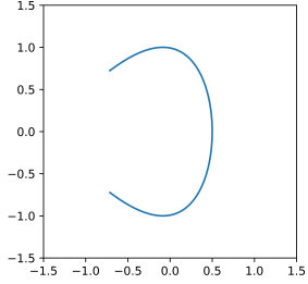
Figure 1: true shape of \Gamma
